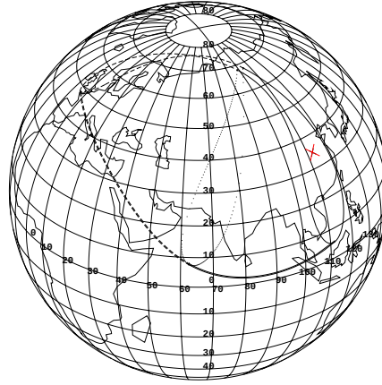
Occultation of Saturn on 513 8 22
