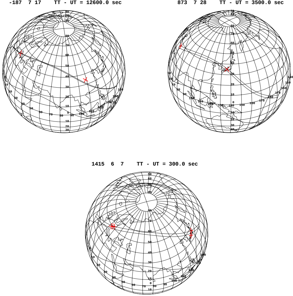
Figure 2: Eclipse bands of the three eclipses in BC 188, AD 873, and AD 1415. The eclipse of BC 188 was observed at Rome and Chang-an (長安). The eclipse of AD 873 was observed at Nishapur and Kyoto (京都). The eclipse of AD 1415 was observed at Aizu (会津), Neider Alteich, Prague, and Wroclaw as total. In Kyoto (京都), it was observed as partial.
