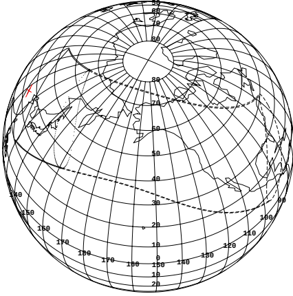
Occultation of Venus on 503 8 5
