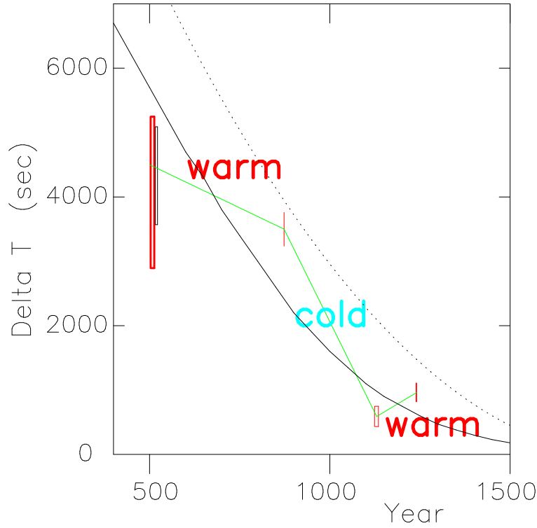
Figure 7: \Delta T variations and Climate.
