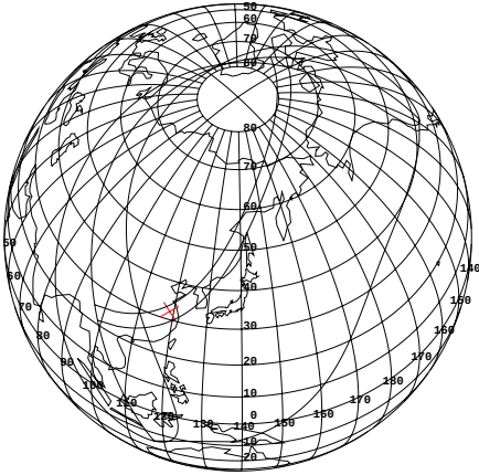
Figure 4: The occultation of Venus on AD 503.08.05 at Luoyang (洛陽). The occultation of Saturn on AD 513.08.22 at Luoyang (洛陽). \Delta T = 4500 sec. Moonrise. Eclipses on 516.04.18 at Jiankang (建康). Eclipses on 522.06.10 at Jiankang (建康). \Delta T = 4500 sec.
