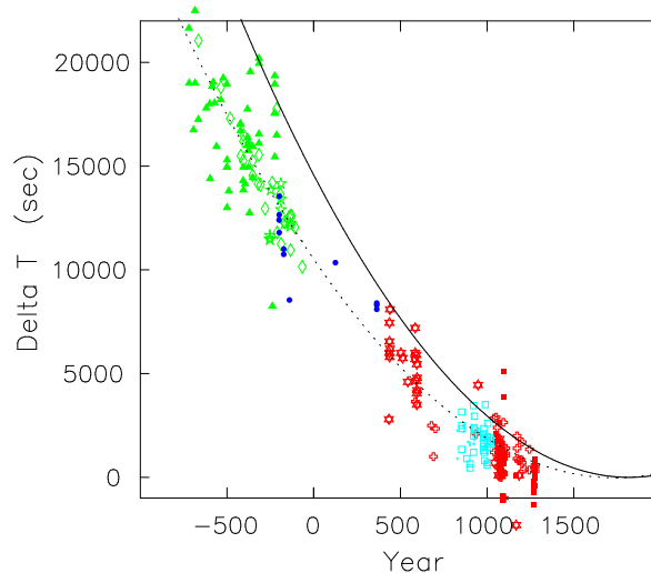
Figure 1: \Delta T variations. The solid curve represents the \Delta T curve predicted by conservation of angular momentum of the Earth-Moon system. The dotted curve is the cubic spline fitting to \Delta T due to Stephenson (1997). Timed lunar and solar eclipses are highly weighted.
