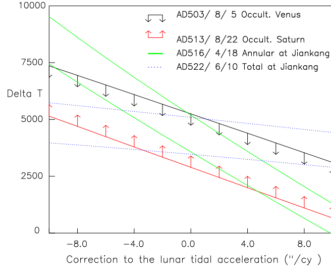
Figure 5: The range of \Delta T from the Sôma Diagram for the years AD 503, 513, 516, and 522.
