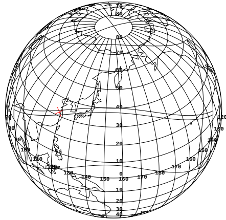
Figure 4: The occultation of Venus on AD 503.08.05 at Luoyang (洛陽). The occultation of Saturn on AD 513.08.22 at Luoyang (洛陽). \Delta T = 4500 sec. Moonrise. Eclipses on 516.04.18 at Jiankang (建康). Eclipses on 522.06.10 at Jiankang (建康). \Delta T = 4500 sec.
