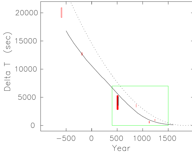
Figure 6: \Delta T variations. The dotted curve corresponds to the conservation of angular momentum of the Earth–Moon system. Solid curve: the cubic spline fitting due to Stephenson (1997). Vertical bars show our results.
