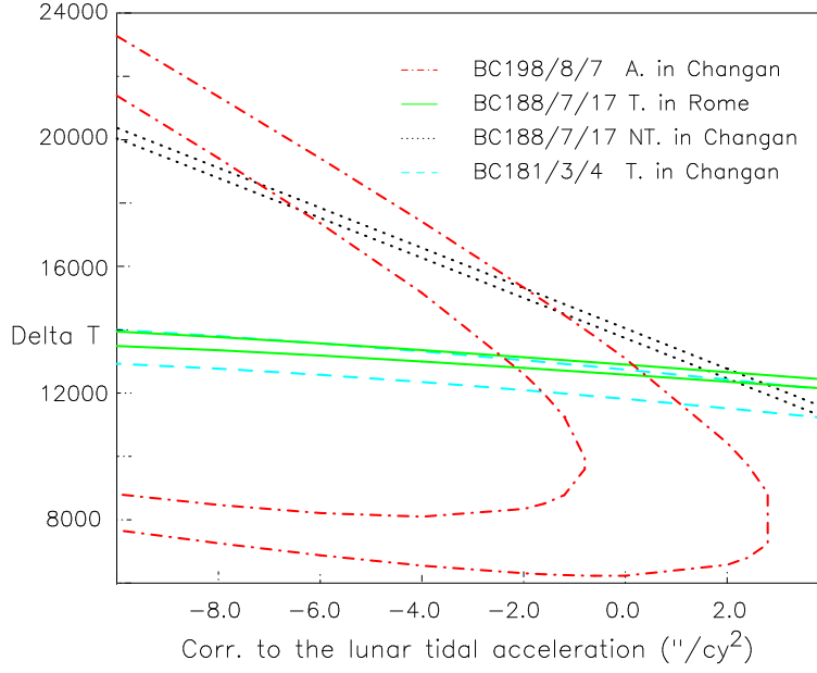
Figure 3: The Sôma diagram for the years BC 198, 188, and 181.
